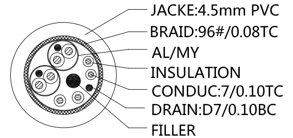
CABLE SPECIFICATION
